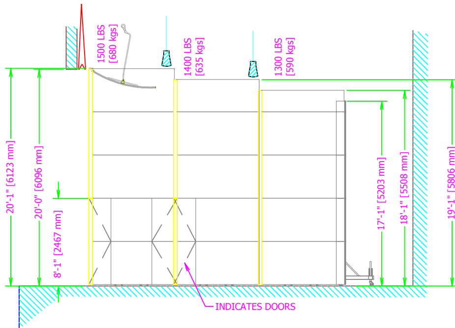
SECTION THRU CENTERLINE
