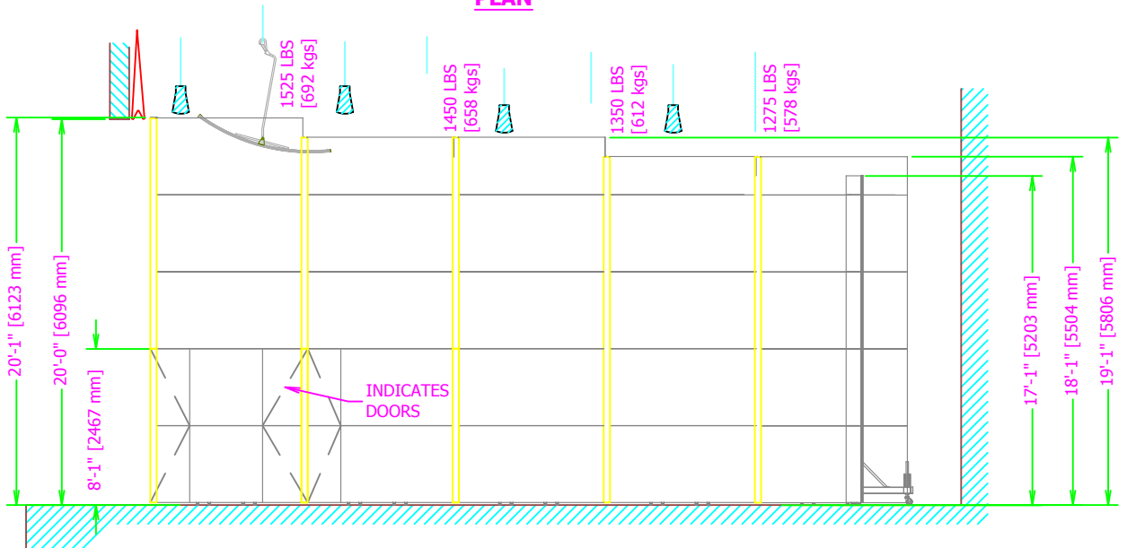
SECTION THRU CENTERLINE
