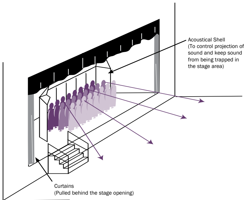
Figure 14 Portable Shell
